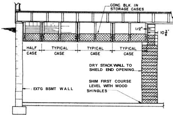
SECTION A-1
