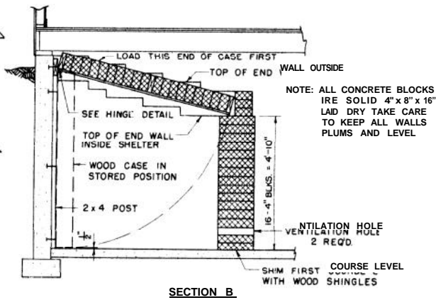
SECTION B
