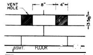
AIR VENT DETAIL
