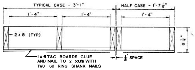
DETAIL SECTIONS
